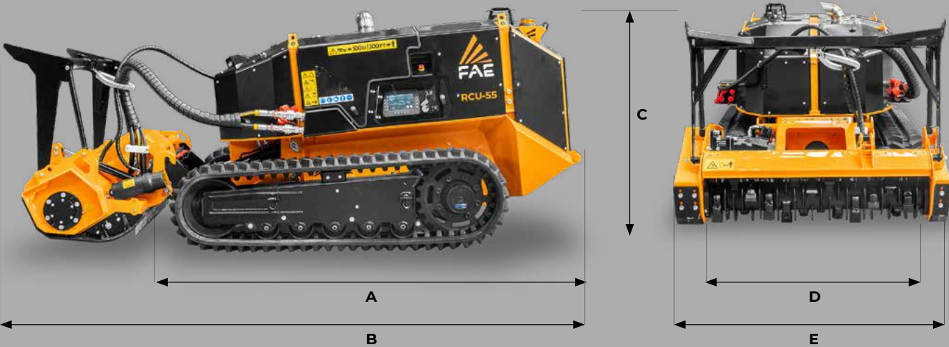
A Overall lenght without attachment B Transport lenght with BLI/RCU attachment on ground 92 in 128 in C Max height D Overall track width E See attachements table 57 in 57 - 69 in
